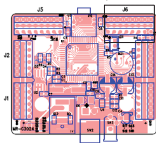
Robonova Controller Board 3024
