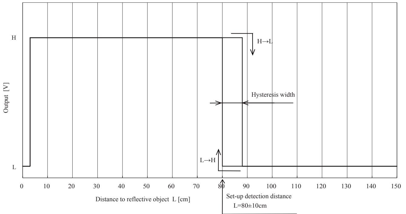
Fig. 2 Example of distance measuring characteristics (output)
